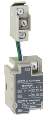
SDx relay module with its terminal block
