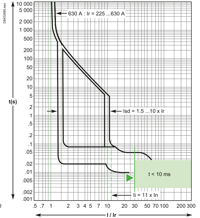
MicroLogic 2.3, 4.3 (up to 570 A) - 630 A
