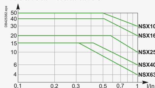
Circuit breaker + motor-mechanism module, in thousands of operations, at 440 V
