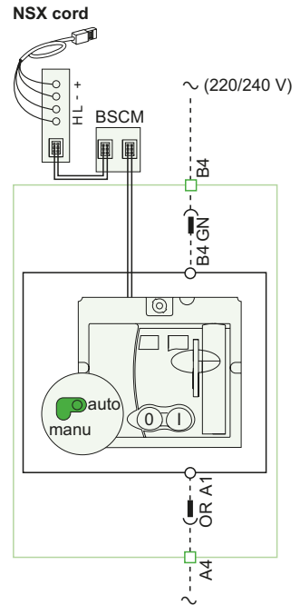
Communicating motor mechanism (MTC)
