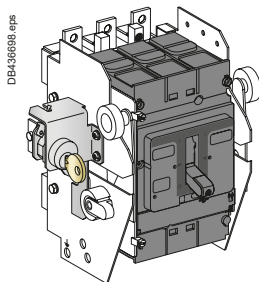
Motor-mechanism locking using a padlock or a keylock
