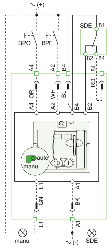
Motor mechanism (MT)
