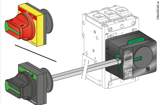
Side mounted rotary handle
