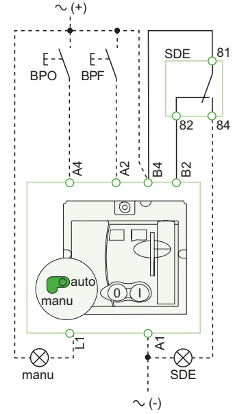
Motor mechanism (MT)
