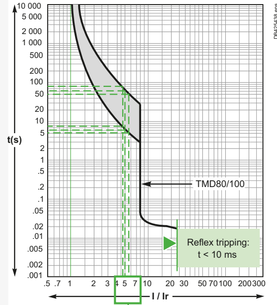
Example 1. Fault I = 500 A
