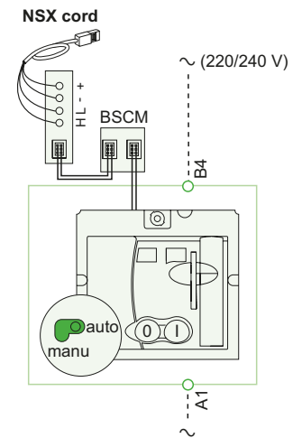
Communicating motor mechanism (MTC)
