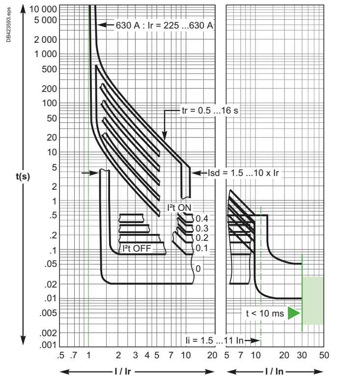
MicroLogic 5.3 and 6.3 E and 7.3 E (up to 570 A) - 630 A
